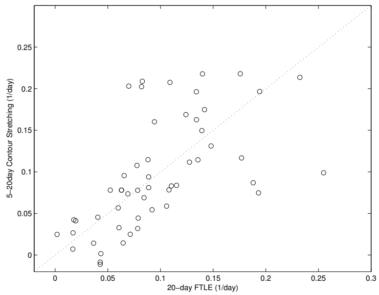
Figure 3: Scatter plot of stretching rate of circular contour (over days 5 to 20) versus 20-day \lambda , for calculations initialized at different locations on 19 November 1997.
