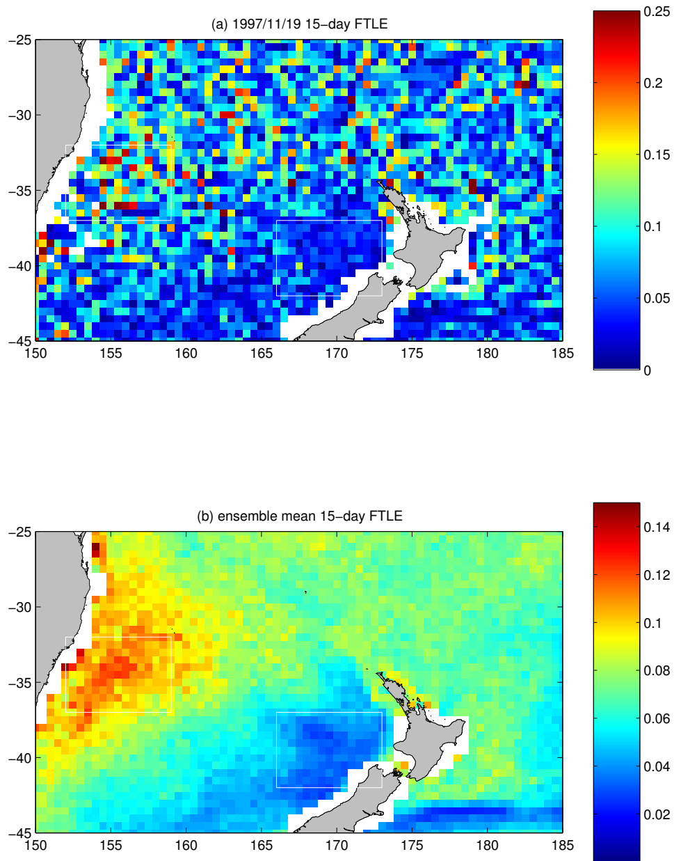
Figure 4: Map of 15-day \lambda for (a) a single calculation for 19 November 1997 and (b) ensemble mean of 108 calculations initialized between 1993 and 2001. Units are \text{day}^{-1} . The white regions correspond to locations where trajectories leave the regions where velocities are defined (e.g. encounter coastal regions) within 15 days, and \lambda cannot be calculated. White boxes are subregions used in later analysis (see text).
