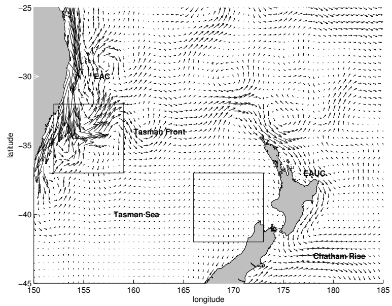
Figure 1: Map of study region showing locations mentioned in the text. Boxes show subregions used in the analysis (see text for details). Vectors are surface velocities derived from the CARS climatology.
