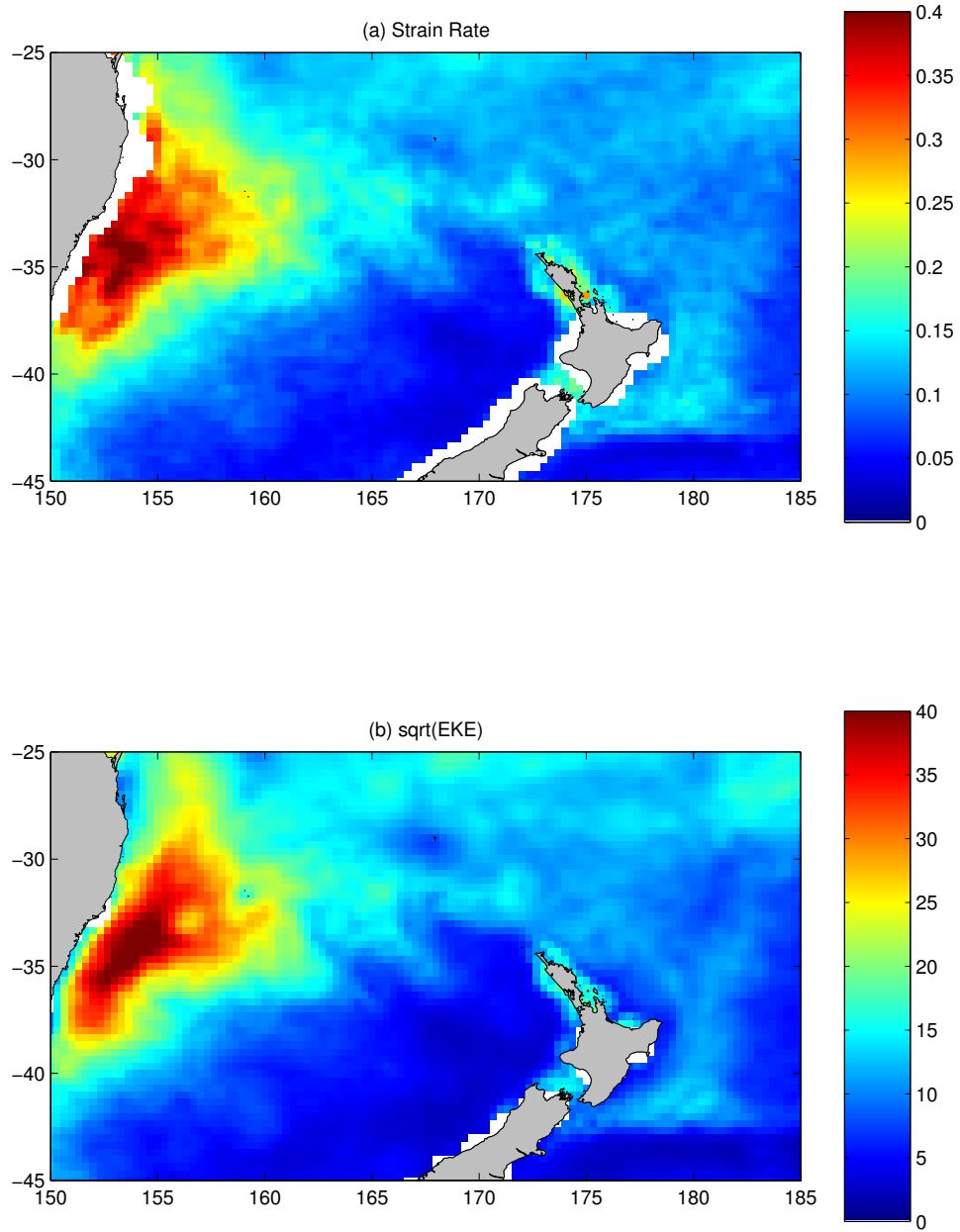
Figure 9: Maps of time-mean (a) strain rate \bar{\gamma} (units 1/day) and (b) EKE^{1/2} (units cm/s).
