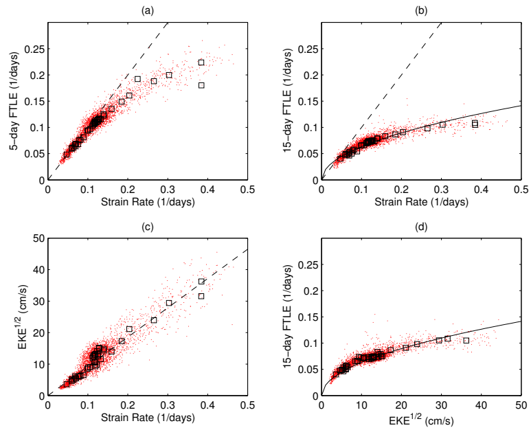
Figure 10: Scatter plots of mean (a) 5-day and (b) 15-day FTLE \bar{\lambda} versus mean strain rate \bar{\gamma} , (c) EKE^{1/2} versus \bar{\gamma} , and (d) 15-day \bar{\lambda} versus EKE^{1/2} . The dots represent individual grid points, while the boxes correspond to averages over all grid points in 5^\circ by 5^\circ subregions. Dashed line in (a) is the 1:1 line, Solid curves in (b) and (d) are quadratic fits to individual points, and dashed line in (c) is EKE^{1/2} = L\bar{\gamma} , with L = 80 km.
