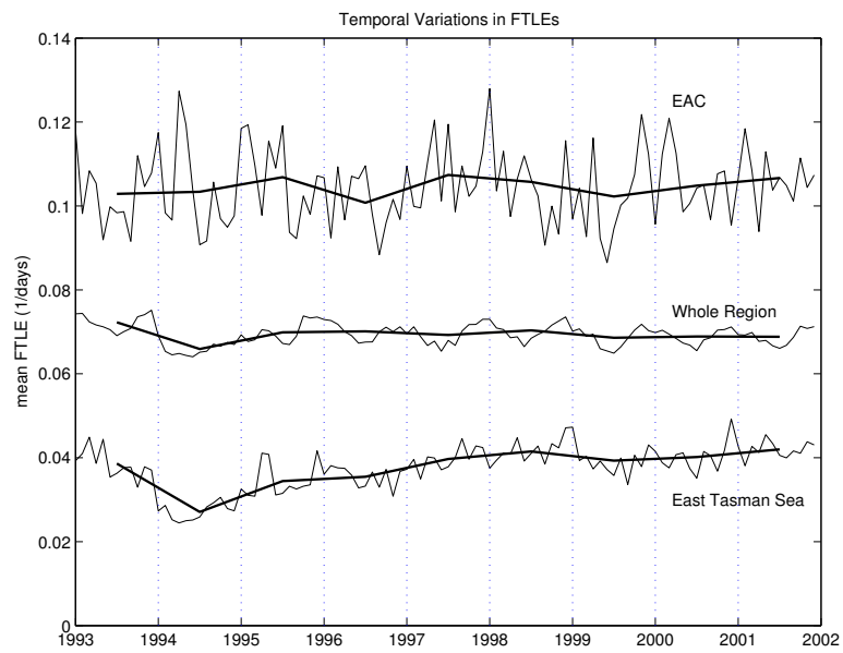
Figure 7: Variation of spatially-averaged 15-day \lambda with date for whole region (middle curve), and for EAC (upper) and east Tasman Sea (lower) regions shown in Figure 1. Thin curves correspond to \lambda for each calculation initialized at the first of each month, and thick curves correspond to the annual mean \lambda (averages over 12 calculations per year).
