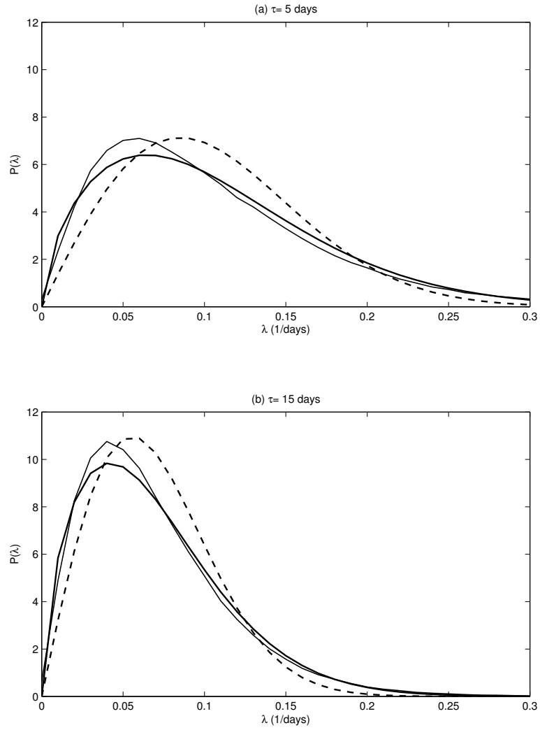
Figure 8: PDFs of \lambda for integration periods of (a) \tau = 5 and (b) 15 days (thin curves), together with Weibull distributions with b = 1.6 (thick solid) and Rayleigh distributions (thick dashed) with the same mean.
