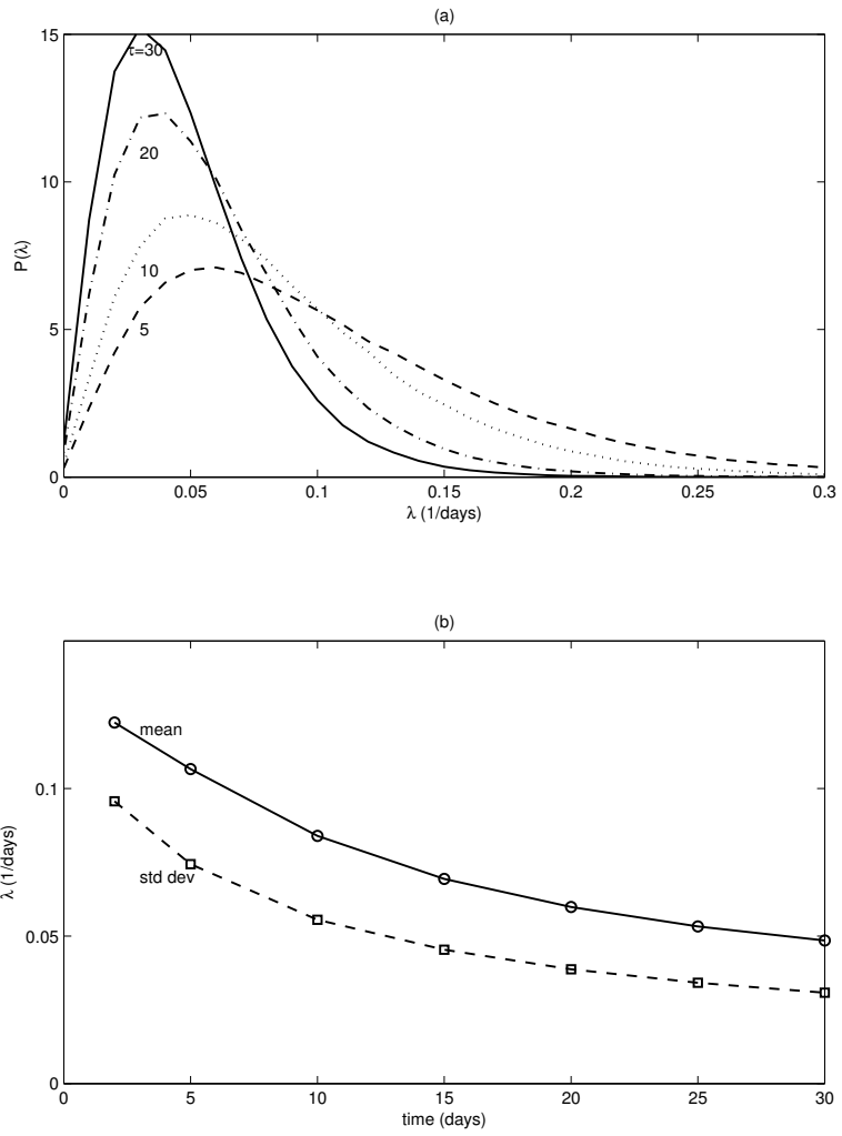
Figure 5: (a) PDFs of \lambda for integration periods of \tau = 5, 10, 20, and 30 days, and (b) variation of mean and standard deviation of \lambda distributions with \tau .
