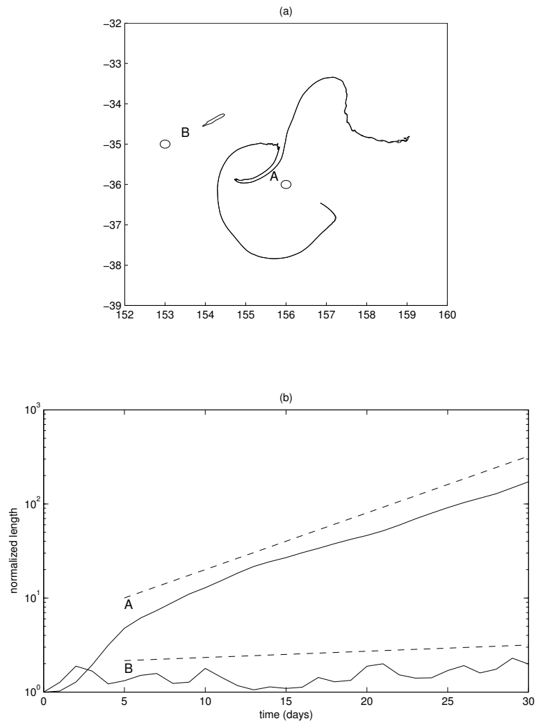
Figure 2: (a) Maps of contours for initial location (circles) and t = 20 days for two different initial locations, on 19 November 1997. (b) Variation of normalized length of contours shown in panel (a) with time. Dashed lines are fits over days 5 to 30.
