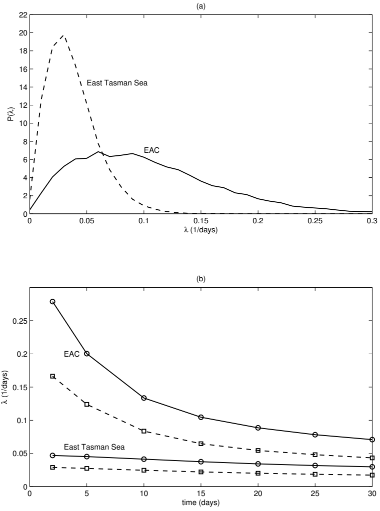
Figure 6: As in Fig. 5 except for the EAC and east Tasman Sea subregions (shown in Fig. 4).
