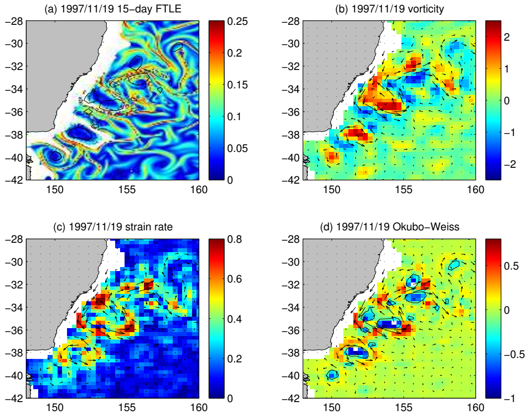
Figure 11: Maps of (a) 15-day \lambda , (b) vorticity \omega , (c) strain rate \gamma , and (d) Okubo-Weiss parameter Q for 19 November 1997. Vectors are surface currents, contours in (a) and (d) Q = -0.2\text{day}^{-1} , and units of all fields are \text{day}^{-1} .
